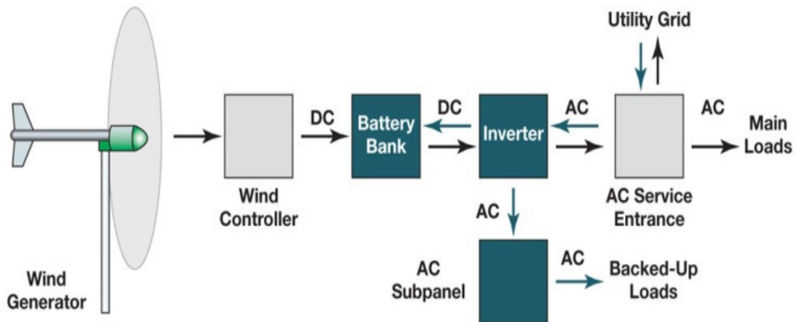
Figure 2: Wind Power System with Back-Up (Source: Home Power online )
