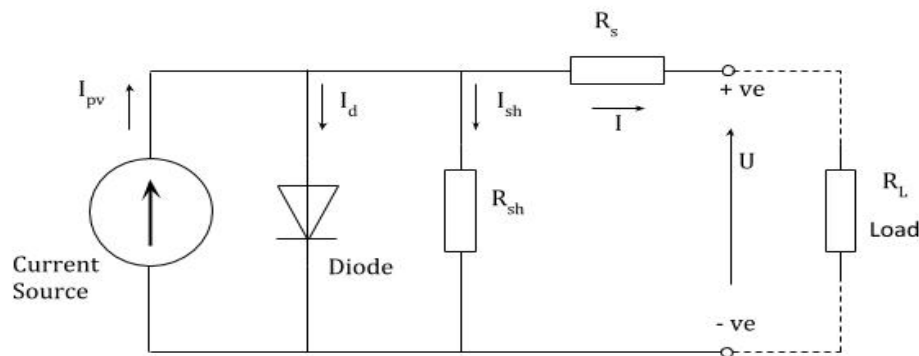
Figure 6: PV Module Equivalent Circuit
