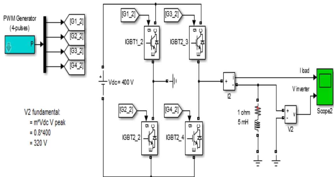
Figure 4: Simulink Model of Full-Bridge Inverter
