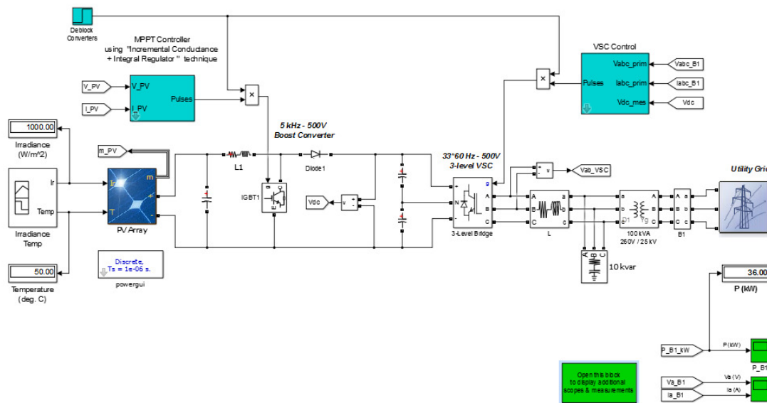
Figure 7: Final 40-kW PV Array with 25-kV Grid Tie-In
