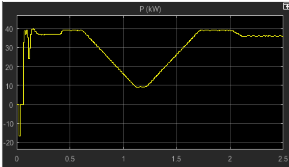
Figure 8: Simulink Scope for P_{out} at T = 2.5s
