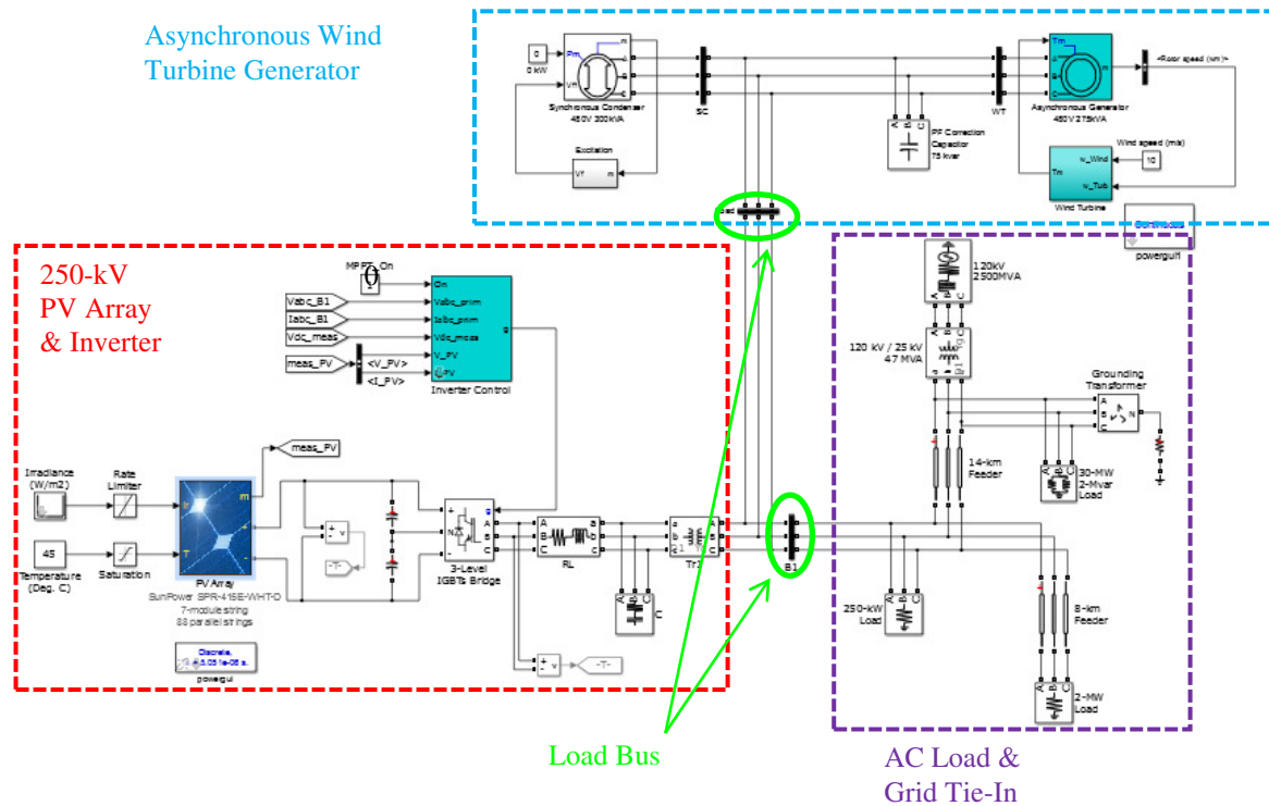
Figure 9: Complete Simulink Model of the Hybrid System
