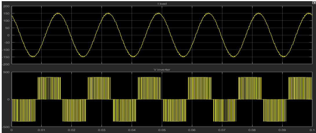
Figure 5: Simulink Scope for Full-Bridge Inverter Output
