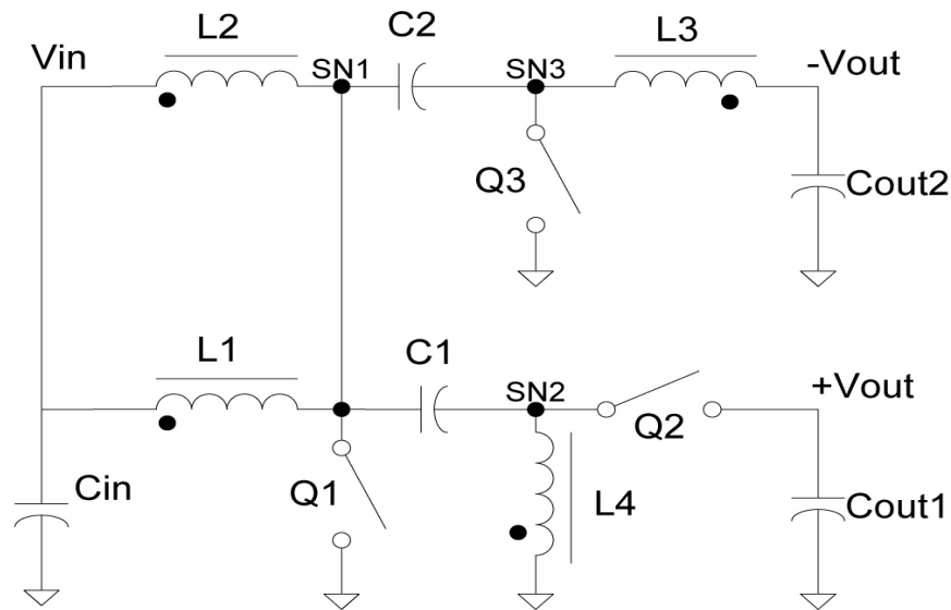
Figure 3: Cuk-SEPIC Circuit Integration (Source: Sumathi, Kumar, and Surekha)
