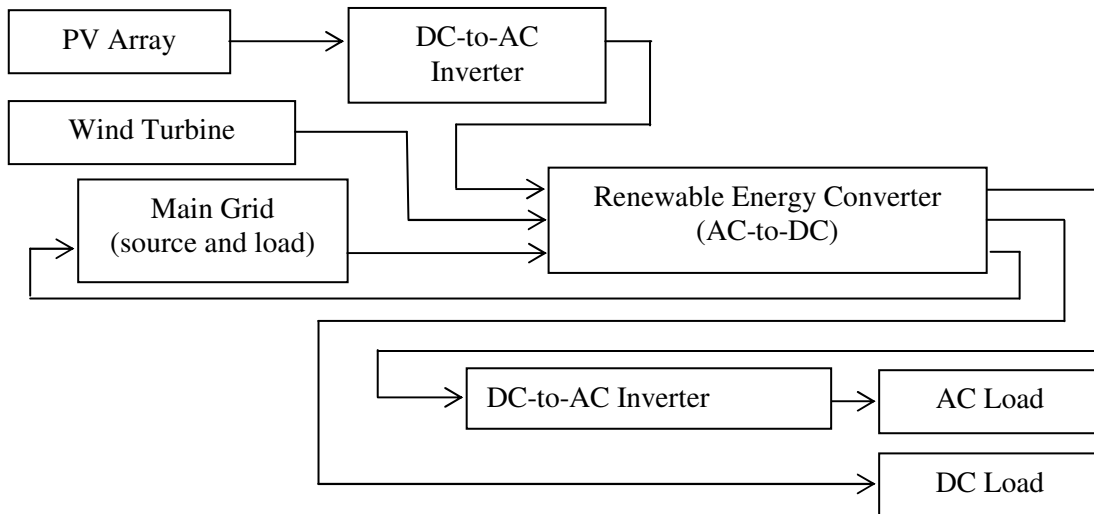
Figure 1: Block Diagram of a Smart Microgrid
